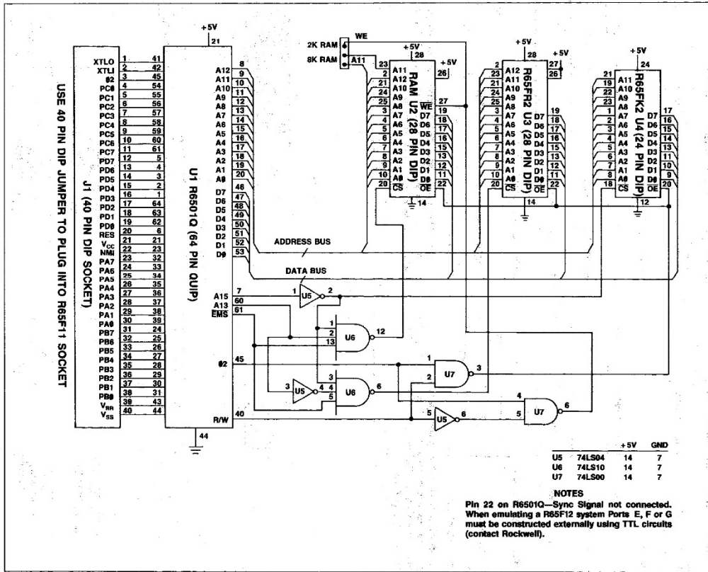
Figure 3. R6501Q, R65FR2 and R65K2 Application Configuration Schematic
